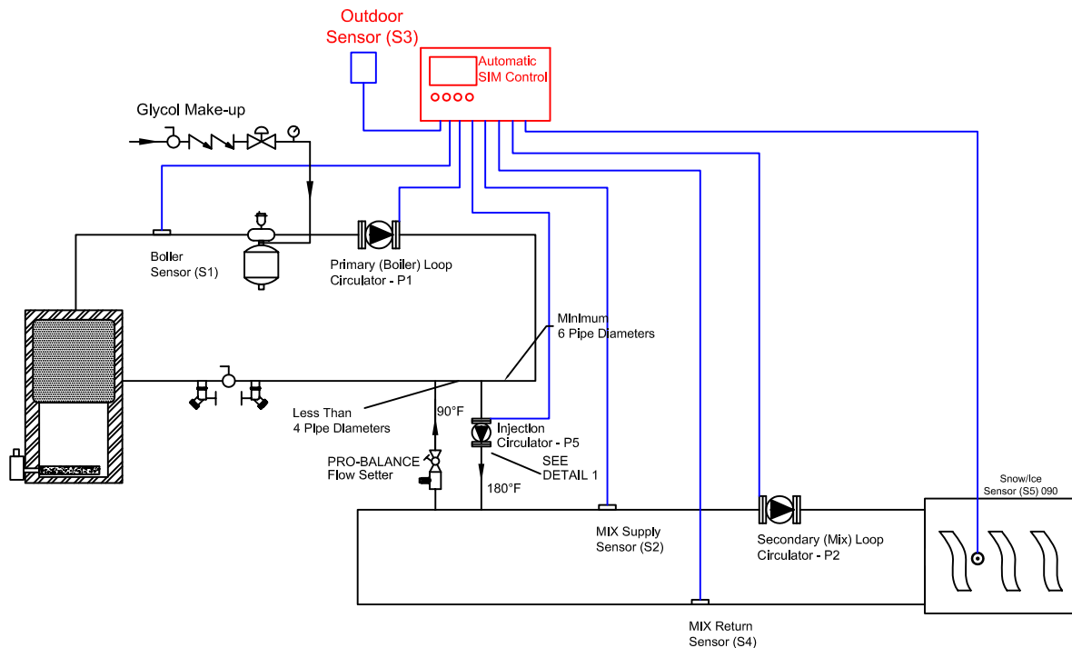
MECHANICAL ROOM SCHEMATIC
