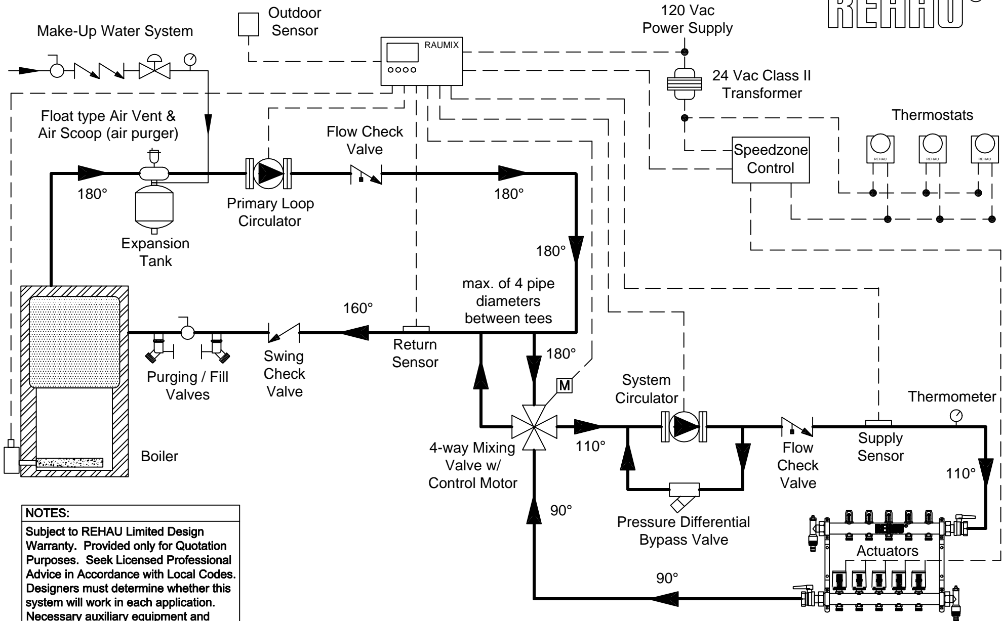
4-Way Mixing Valve w/ Deluxe RFH Mixing Control & Speed Zone Controls
